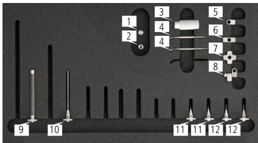
VAST XXT styli Kit 4, small, set of 15 set 626103-9024-000
